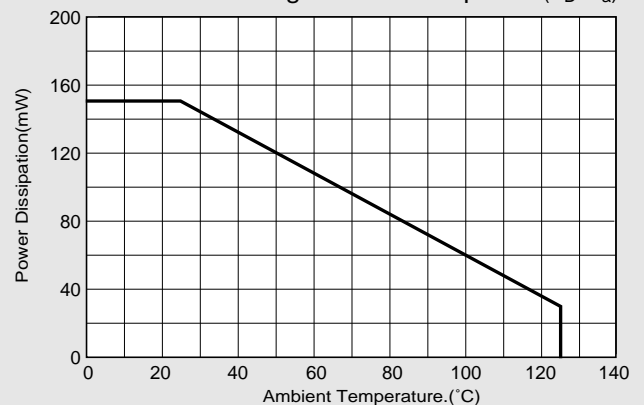
Allowable Package Power Dissipation ( P_D - T_a )
